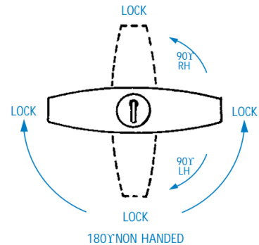
GB7-G00144 (Locking, large T, 38 mm open fixing)
